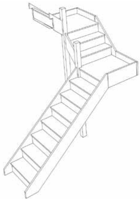
Stair-S7QL2QL1N-LH
