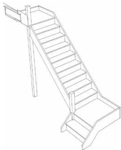
Stair-S1QL8QL1N-LH
