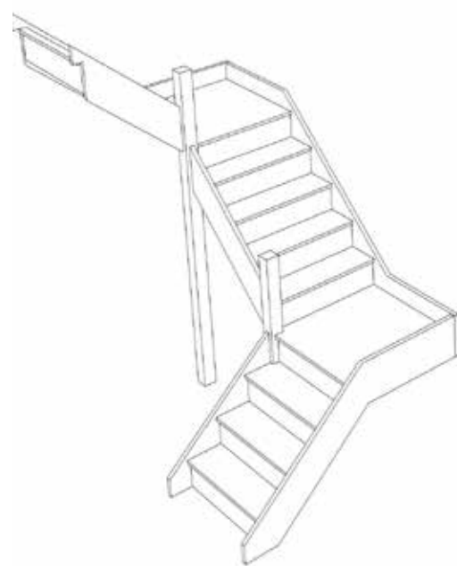
Stair-S3QL4QL3N-LH
