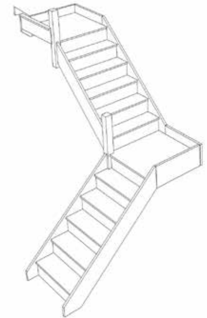
Stair-S5QL5QLN-LH
