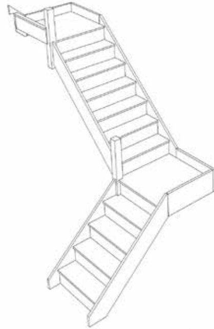
Stair-S4QL6QLN-LH
