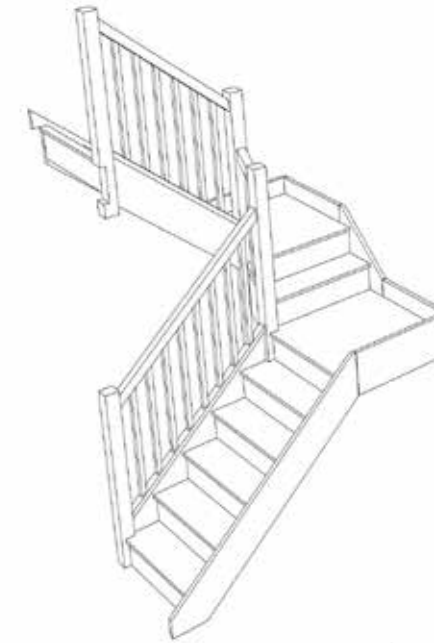
Stair-S5QL1QL4N-LH-HR
