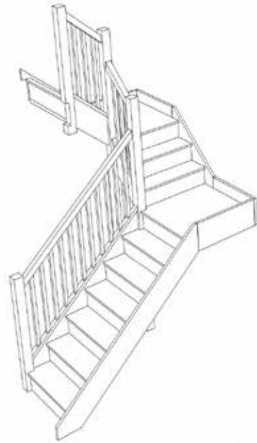
Stair-S6QL2QL2N-LH-HR
