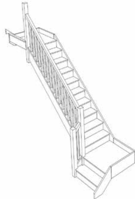
Stair:S1QL9QLN-LH-HR
