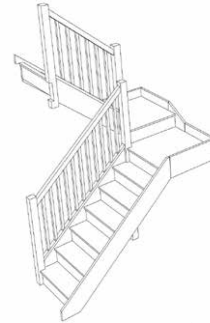
Stair-S6QLQL4N-LH-HR
