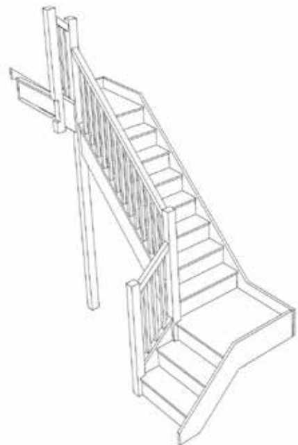
Stair-S2QL7QL1N-LH-HR
