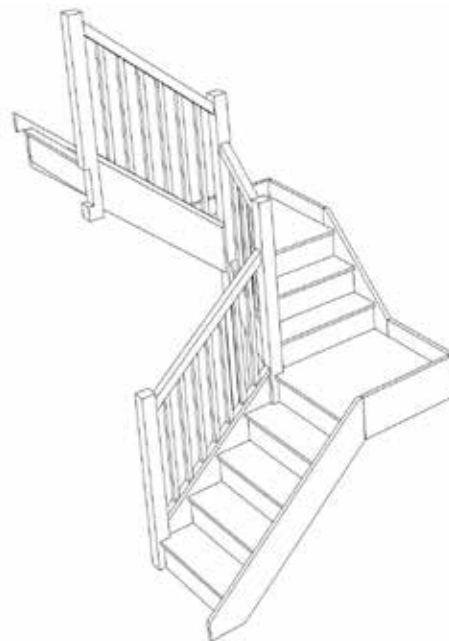
Stair-S4QL2QL4N-LH-HR
