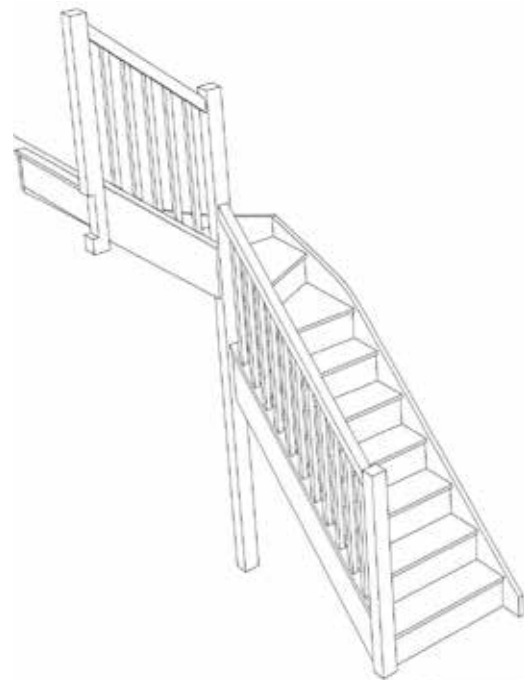
Stair:S6W33N-LH-HR
