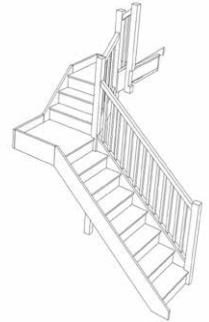
Stair:S7QL2QL1N-RH-HR
