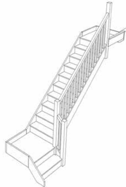
Stair:S1QL9QLN-RH-HR
