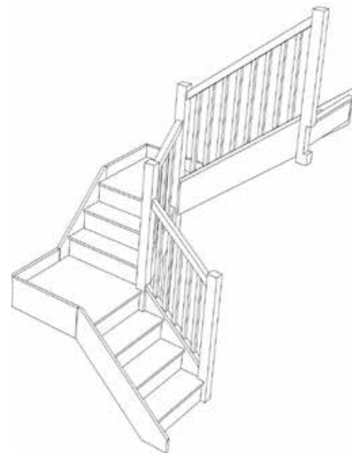
Stair-S3QL2QL5N-RH-HR
