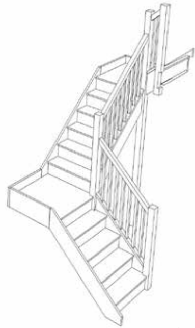
Stair:S4QL5QL1N-RH-HR
