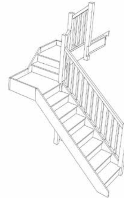
Stair:S7QL1QL2N-RH-HR
