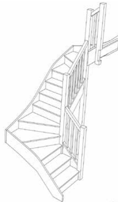
Stair:S2W33W31N-RH-HR
