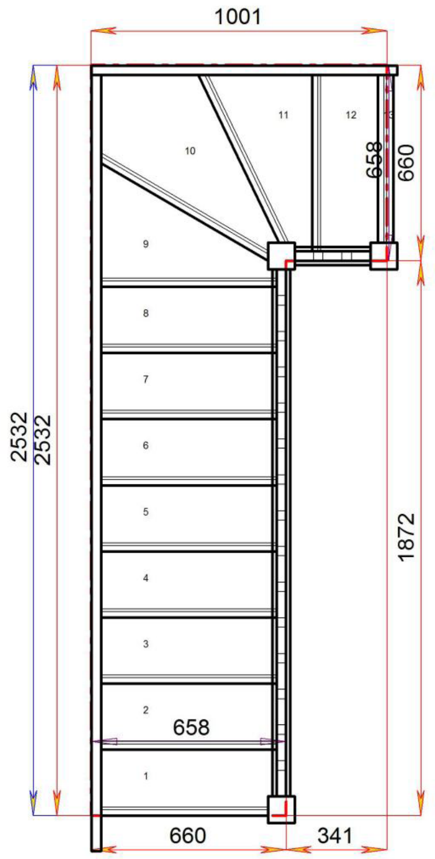
Floor to floor height 2600.000 mm
