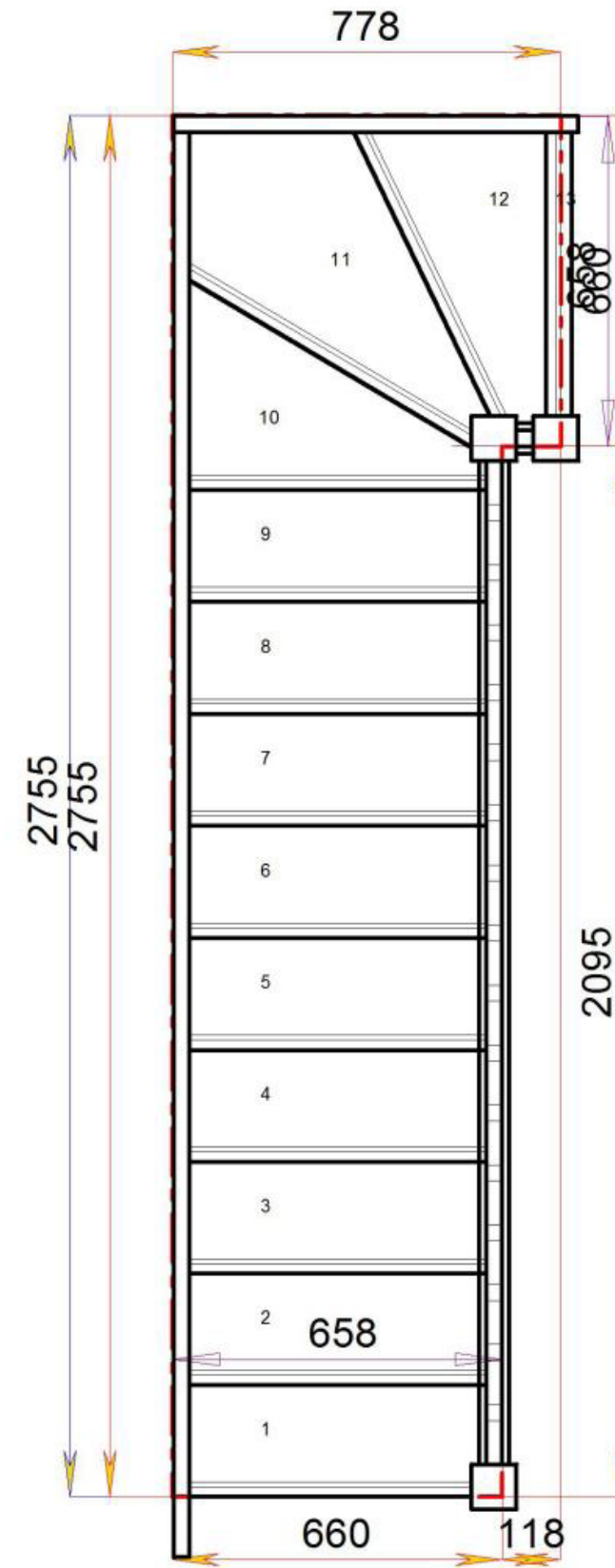
Floor to floor height
