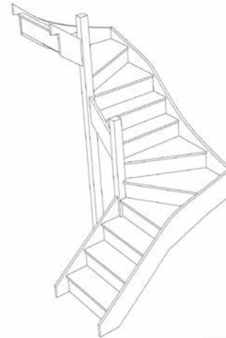
Stair:S3W32W31N-LH
