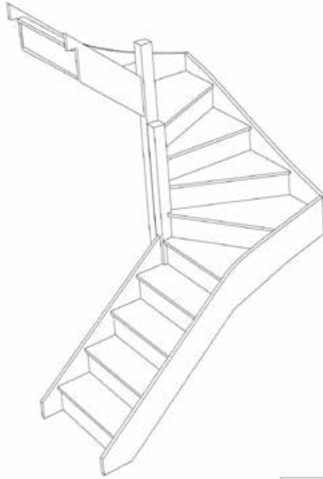
Stair:S4W3W32N-LH
