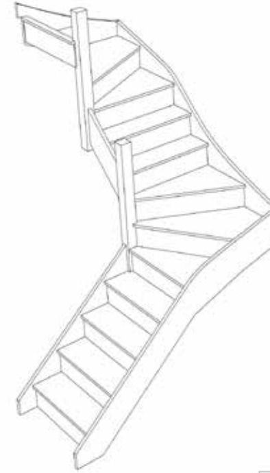
Stair:S4W32W3N-LH
