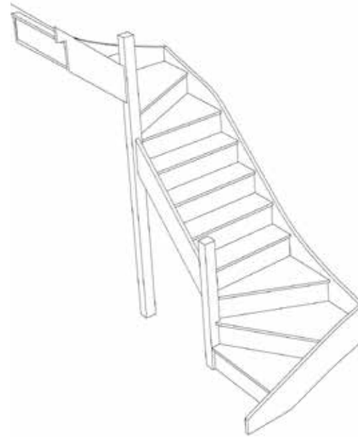
Stair:SW34W32N-LH
