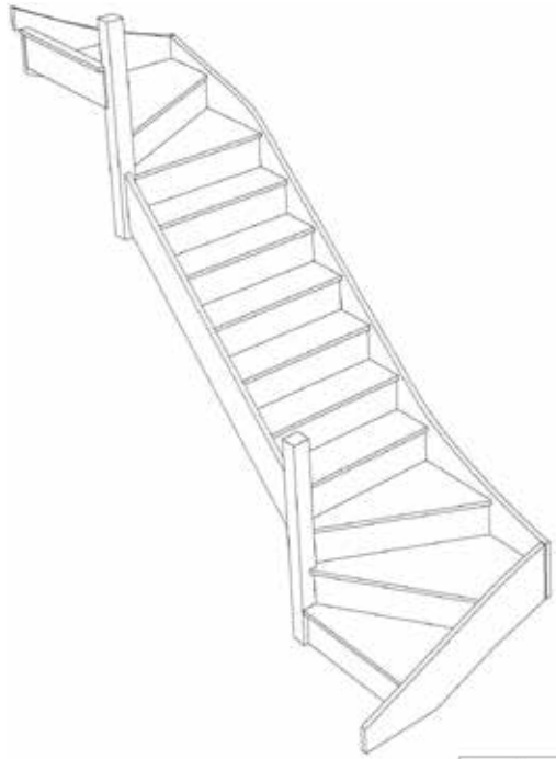
Stair:SW36W3N-LH
