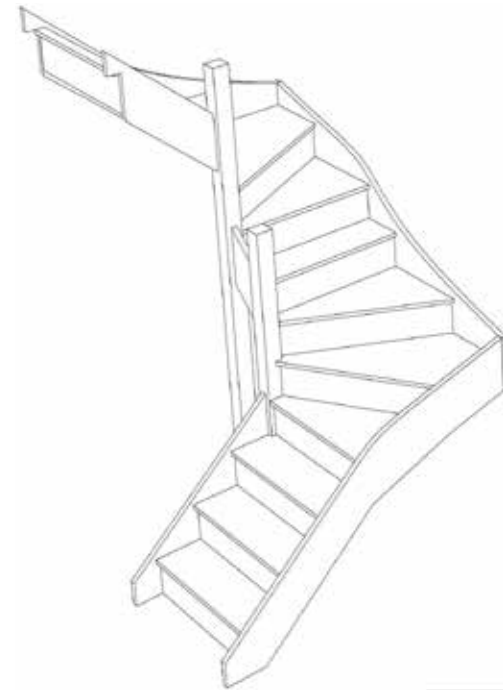
Stair:S3W31W32N-LH
