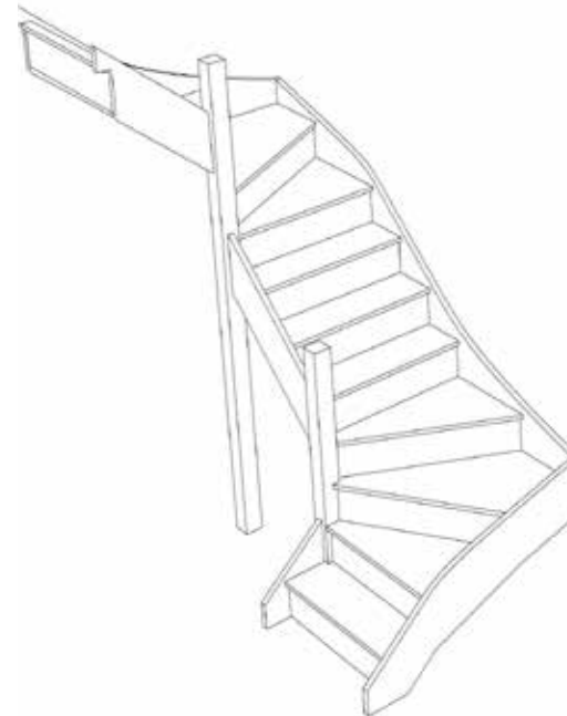
Stair:S1W33W32N-LH
