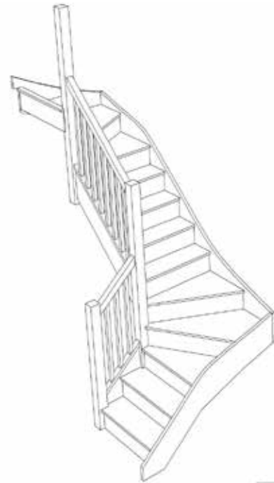
Stair:S2W34W3N-LH-HR
