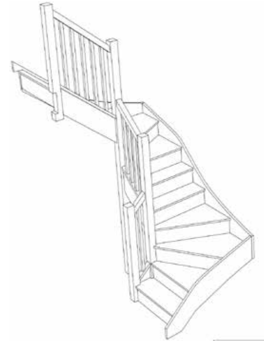
Stair:S1W32W33N-LH-HR
