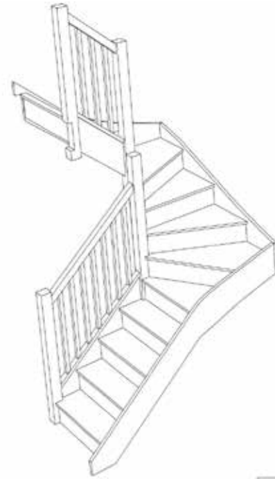
Stair:S4W3W32N-LH-HR
