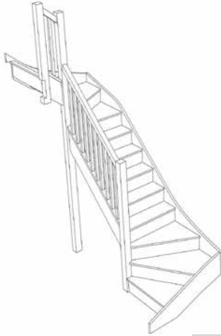
Stair:SW35W31N-LH-HR
