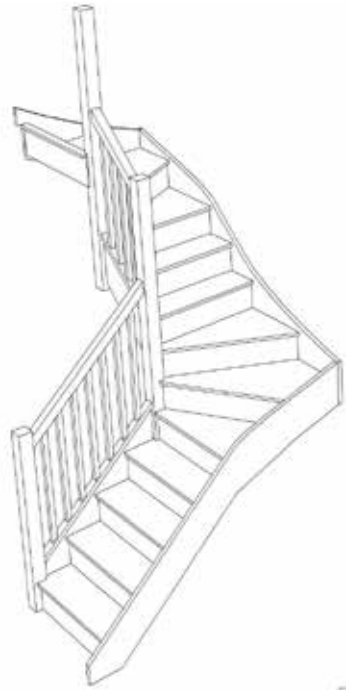
Stair:S4W32W3N-LH-HR
