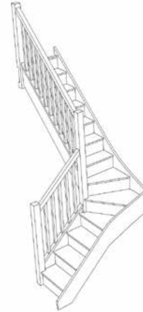
Stair:S3W36N-LH-HR
